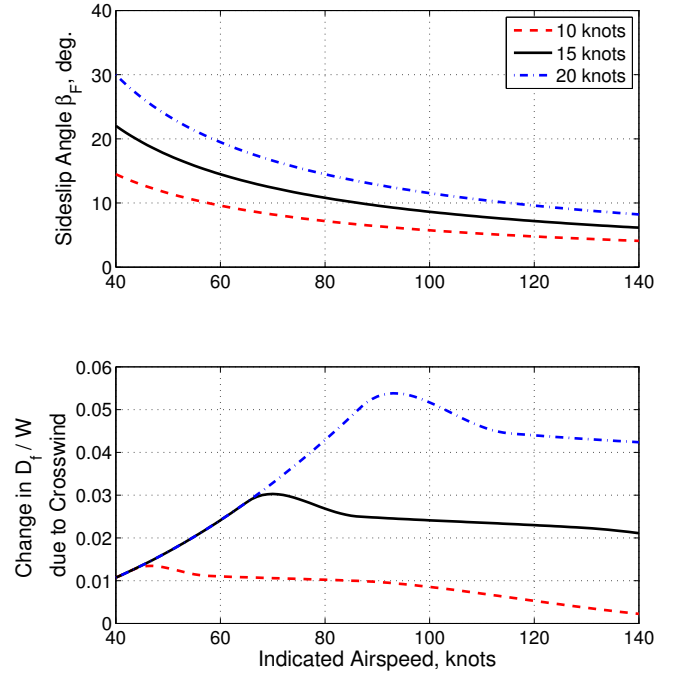
Fig. 5. Change in sideslip angle, \beta_F , and drag-to-weight ratio, D_f/W , as a function of airspeed, V_{IAS} , due to crosswinds of different magnitudes during sideslipped flight.
