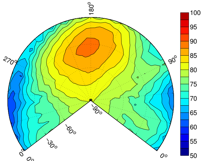
(a) No wind.
