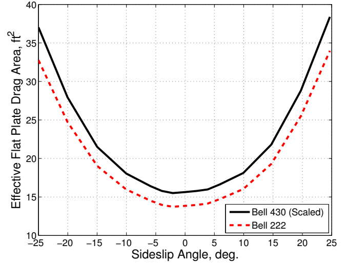
Fig. 3. Fuselage drag variation with sideslip angle for the Bell 430 derived from full scale measurements of the Bell 222 helicopter in the Ames 40'x80' wind tunnel. (Ref. 25)
