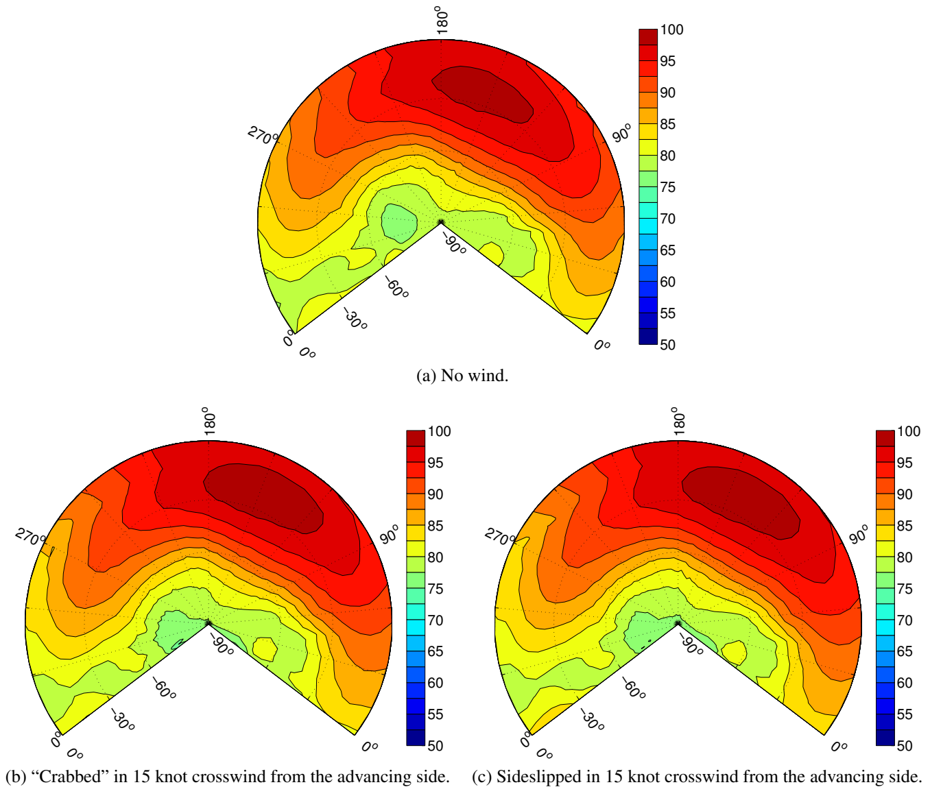
Fig. 10. Predicted overall noise hemispheres for 130 KIAS level flight, dB OASPL.
