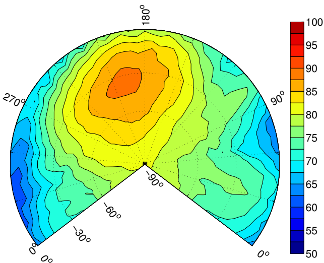
(d) "Crabbed" in 15 knot crosswind from the retreating side.
