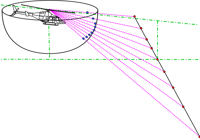
Fig. 1. Diagram of the process of building an empirical source noise hemisphere for a straight-line steady flight condition. Red points represent ground-based microphone locations and blue points the corresponding locations on the acoustic hemisphere surface.
