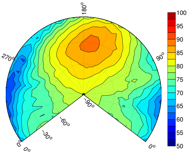
(b) "Crabbed" in 15 knot crosswind from the advancing side.
