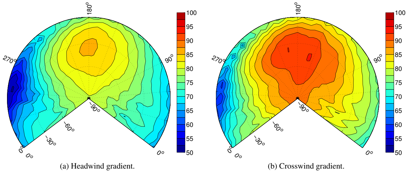
Fig. 12. Predicted BVI noise hemisphere for 80 KIAS, -7.5° FPA flight in a wind gradients, dB BVISPL.
