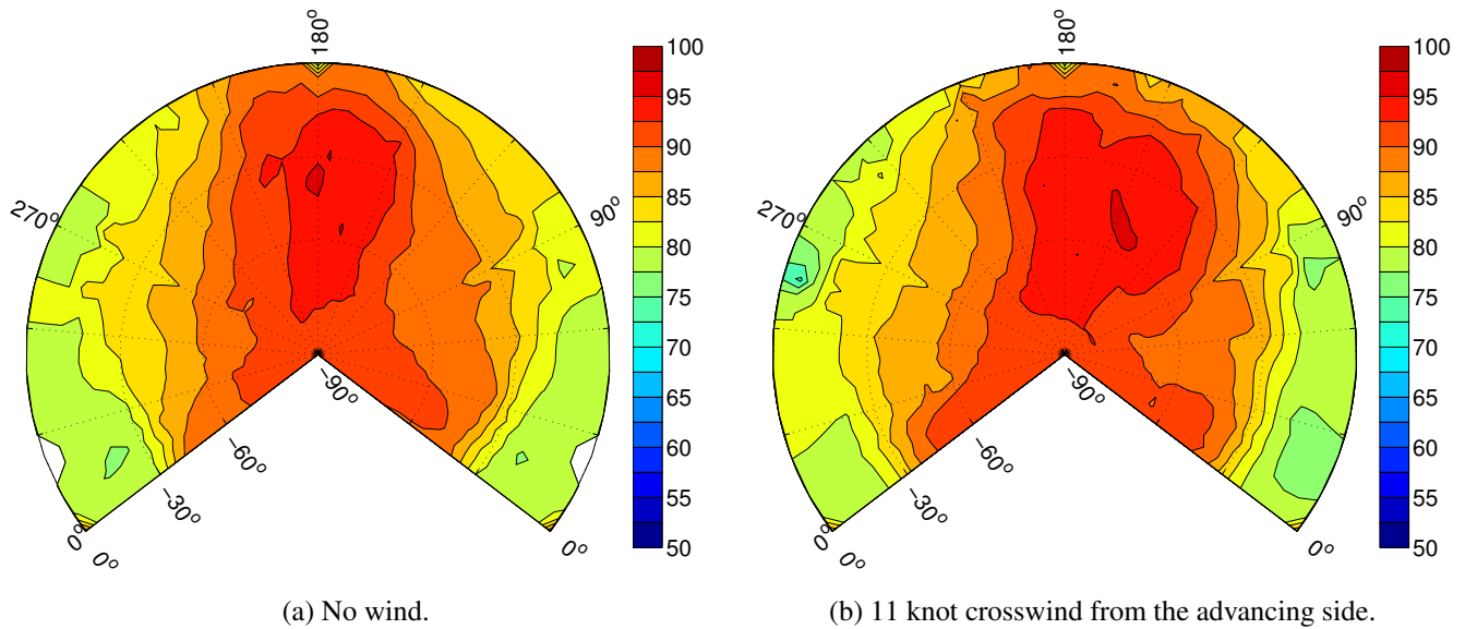
Fig. 6. Measured BVI noise hemispheres for 80 KIAS, -7.5° FPA flight condition, dB BVISPL
