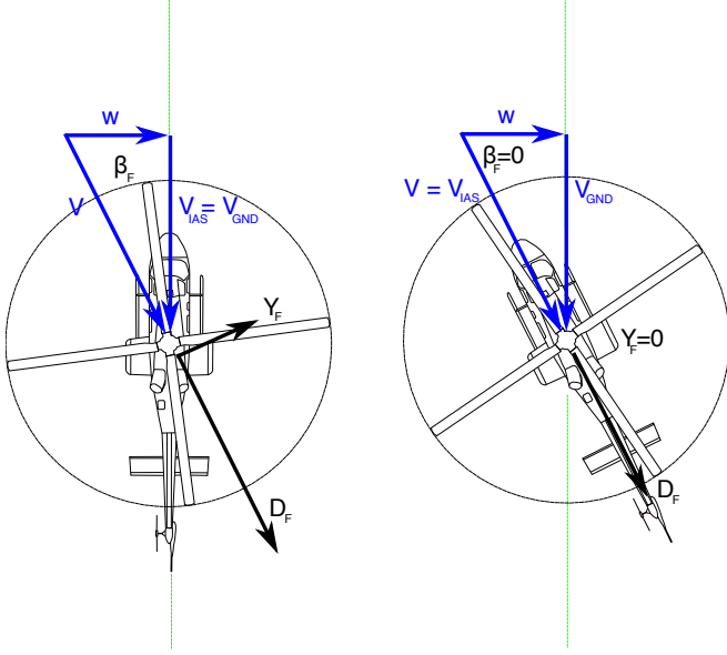
Fig. 4. Top view schematic of helicopter fuselage velocities and forces under crosswind conditions for a) sideslipped flight and b) “crabbed” flight.
