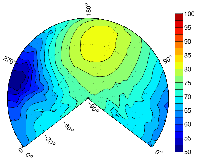
(c) Sideslipped in 15 knot crosswind from the advancing side.
