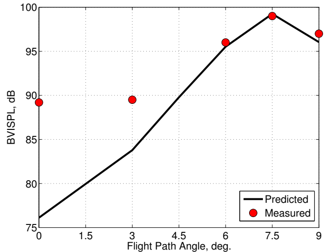
Fig. 9. Comparison of measured and predicted BVISPL at 180^\circ azimuth, -30^\circ elevation at 80 KIAS for various flight path angles.
