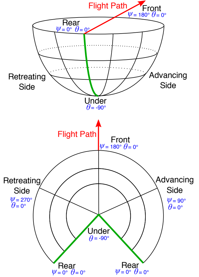
Fig. 2. Lambert projection of an acoustic hemisphere.
