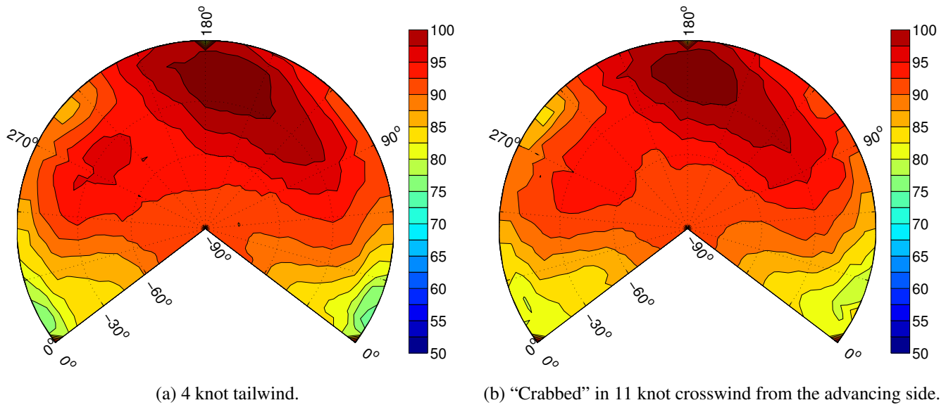
Fig. 7. Measured noise hemispheres for 130 KIAS, level flight, dB OASPL.
